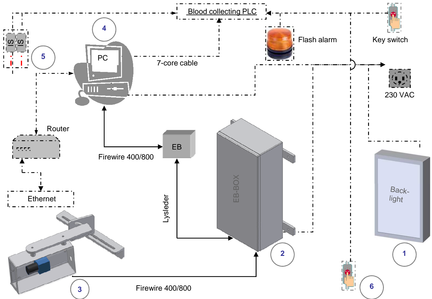
1 = Backlight, 2 = Extender box, 3 = Camera box, 4 = PC, 5 = Inductive sensors, 6 = Alarm receipt button
